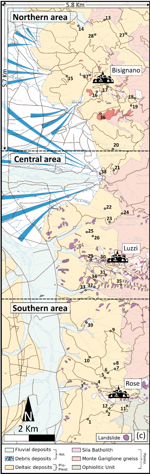
Figure S1: Schematic geological map of the eastern margin of the Crati Basin displaying the location of the measured logs and studied locations. Northern, central, and southern sectors extension are displayed. Modified after Tansi et al. (2016).
