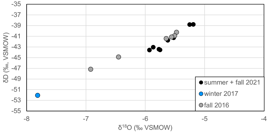
Supplemental 3: Oxygen and hydrogen stable isotope data from all water samples. Measured relative to Vienna Standard Mean Ocean Water.
