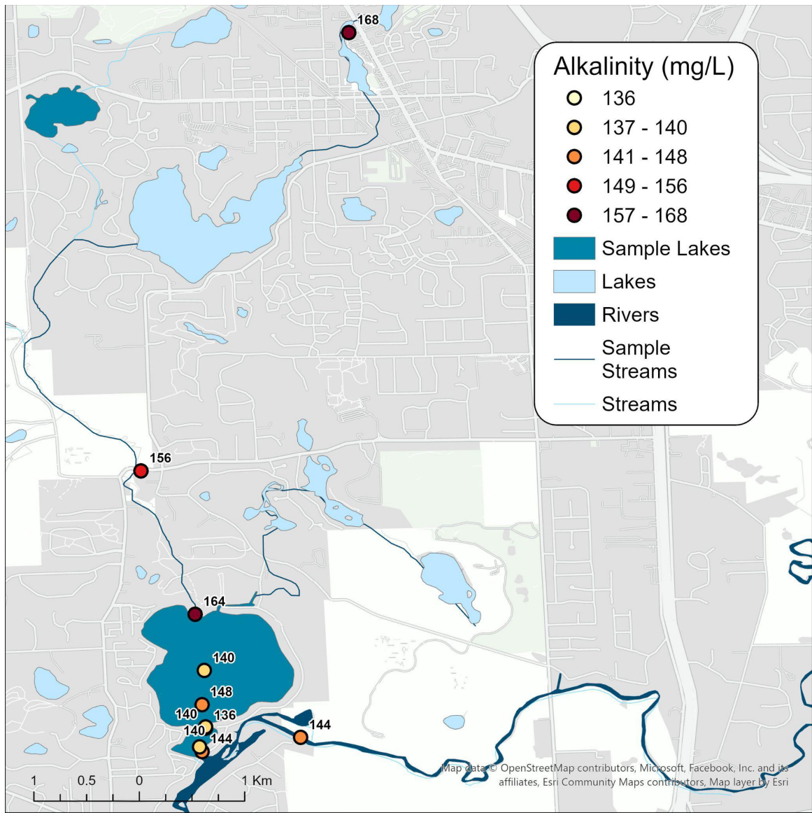
Supplemental 2: Map of recent alkalinity data. Note general decrease in values from north to south.
