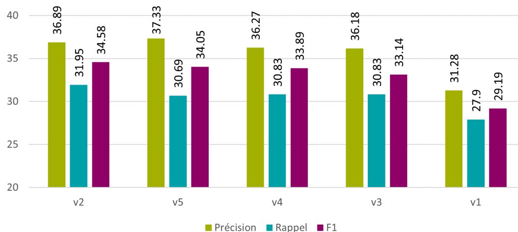
Figure 19 : Tesseract – correction brute – mots
