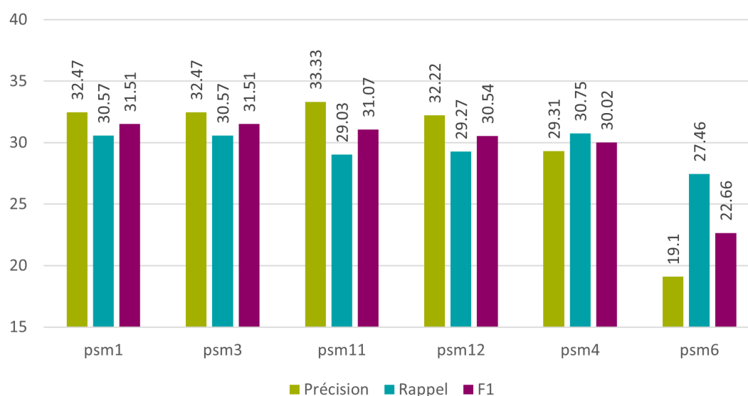
Figure 10 : Tesseract – phase 2 – psm – mots
