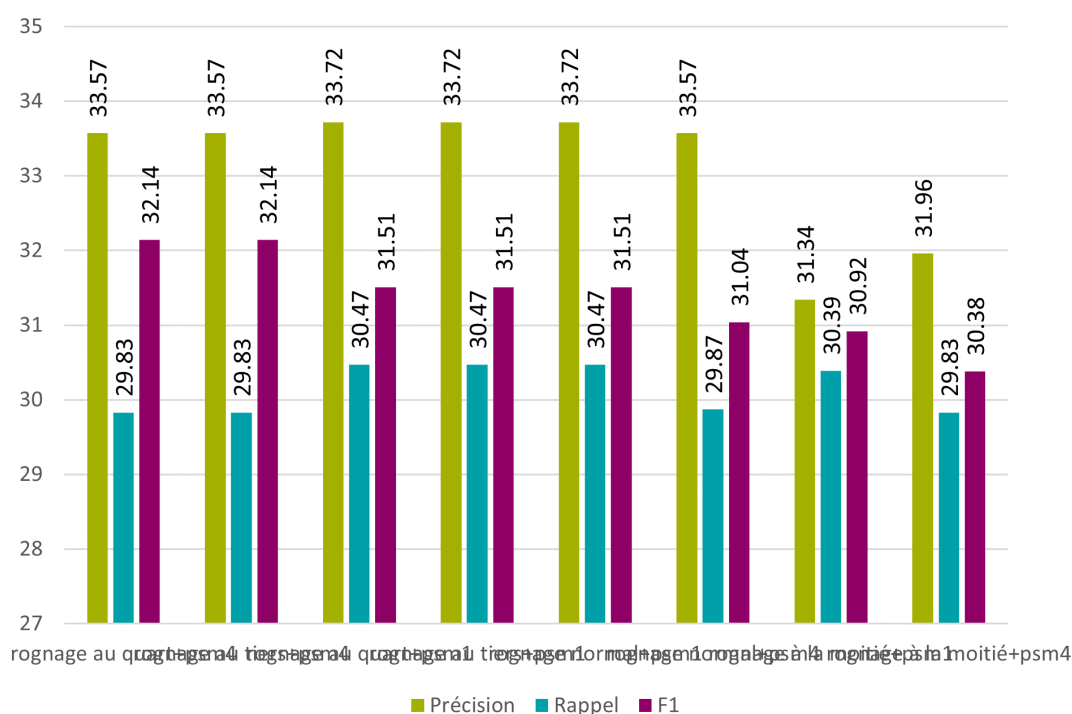
Figure 17 : Tesseract – pré-traitement intelligent – mots
